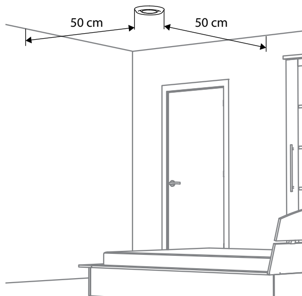
Supply air disk valve location
