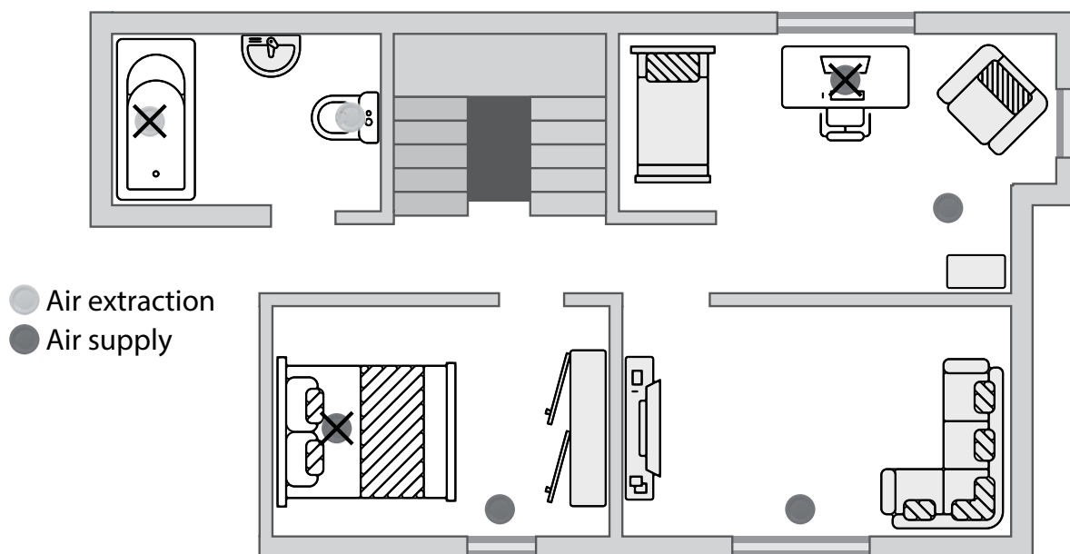
Recommendations on positioning of supply and exhaust grilles
